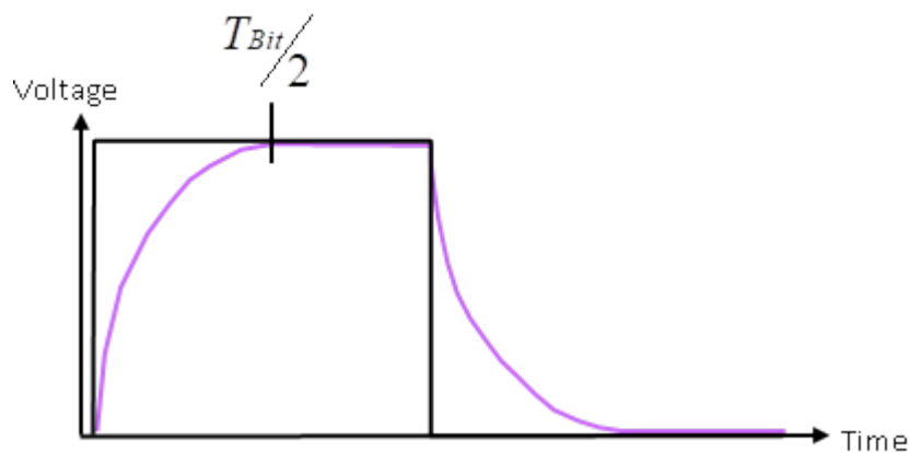
Figure 5-5: Signal waveform for PROFIBUS cables that are too long
