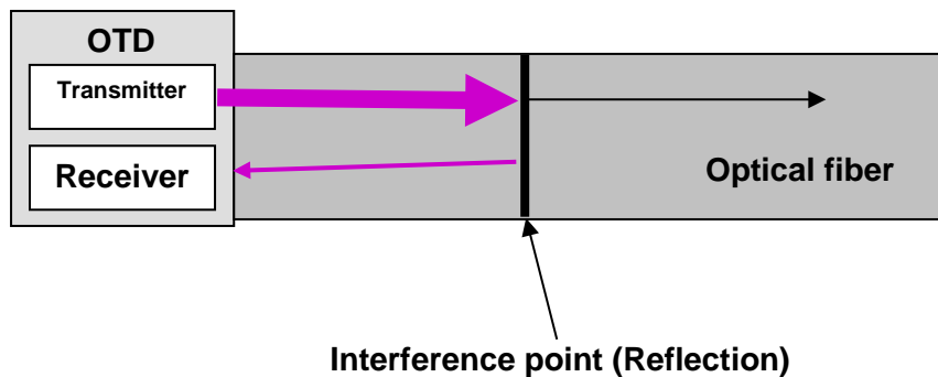
Figure 5-12: OTDR measurement principle
