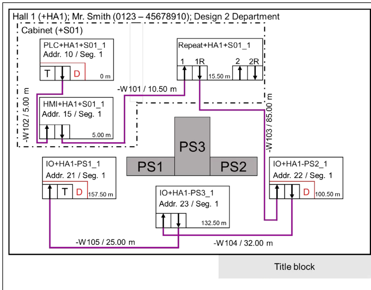
Figure 6-6: Example of PROFIBUS forwards documentation, physical topology plan
