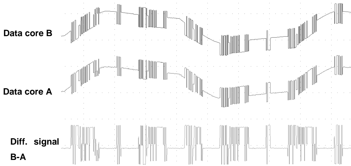
Figure 5-4: Measurement PROFIBUS RS-485
