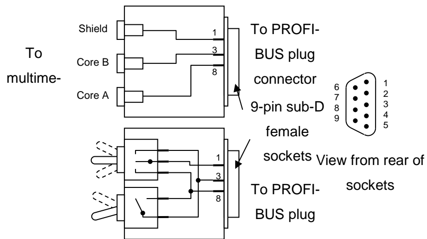
Figure 6-2: Measurement aid sockets (PROFIBUS RS485)
