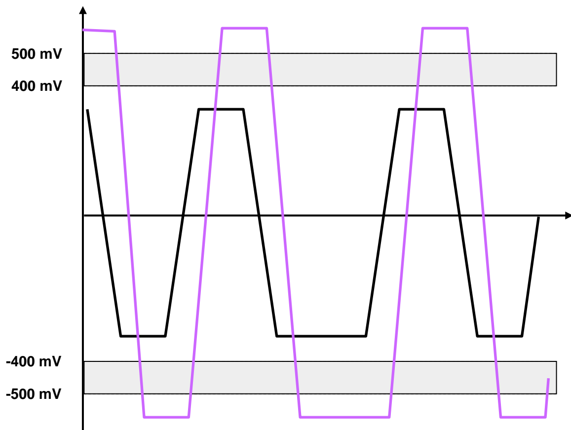
Figure 5-10: PROFIBUS MBP (PA) with defective bus terminator
