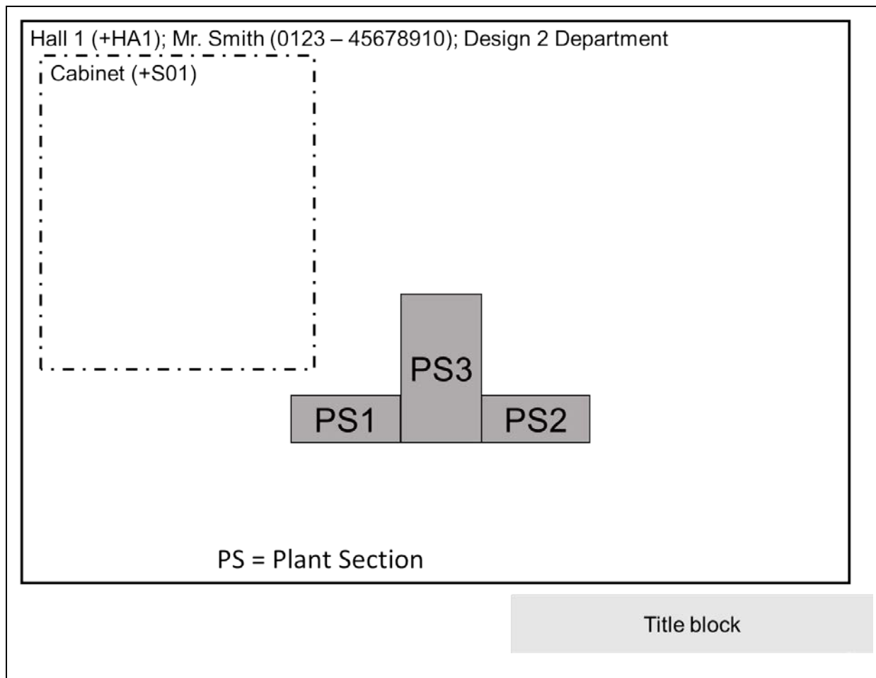
Figure 6-5: Example of forwards documentation for the automation of three plant sections
