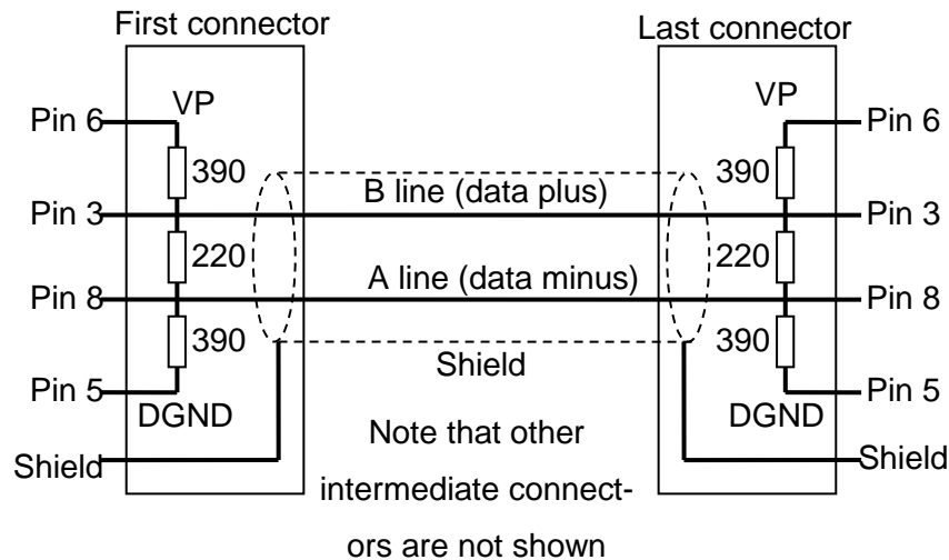
Figure 6-1: PROFIBUS RS485 cable schematic with end terminations switched in
