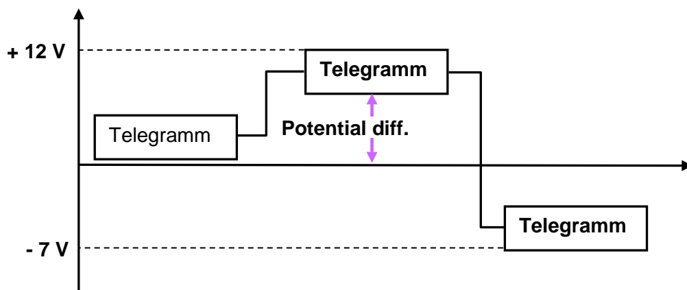
Figure 5-2: Potential shift at signals
