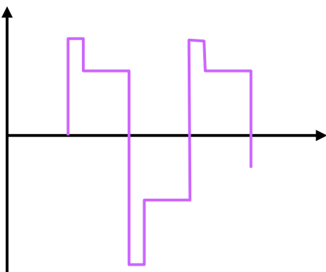
Figure 5-7: Too much terminator resistance
