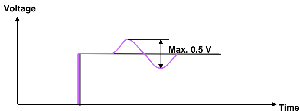
Figure 5-6: Signal waveform for non-connected PROFIBUS stations
