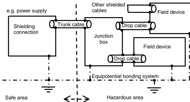
Figure 17: Ideal connection of cable shields to the equipotential bonding
