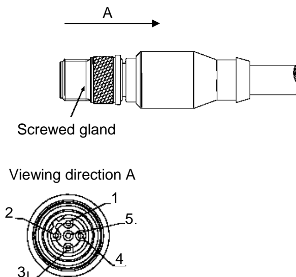
Figure 10: 5 pin M-12 male plug for RS 485
