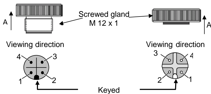
Figure 11: 4-pin M-12 connector (for MBP (PA)) – male plug (left) and female socket (right)
