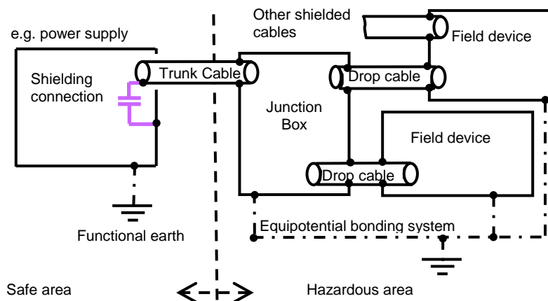
Figure 18: Capacitive earthing for PROFIBUS-MBP (PA)
