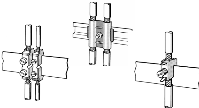
Figure 19: Techniques for connecting the cable shield to equipotential bonding
