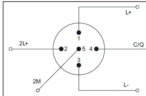
Figure 5: Pin assignment Port Class B
