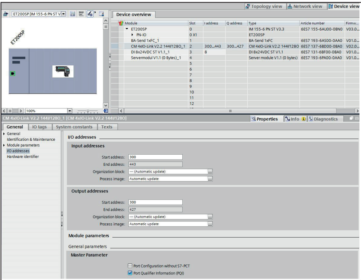
Figure 8: Device view of the PROFINET device with setting of the IO-Link address range
