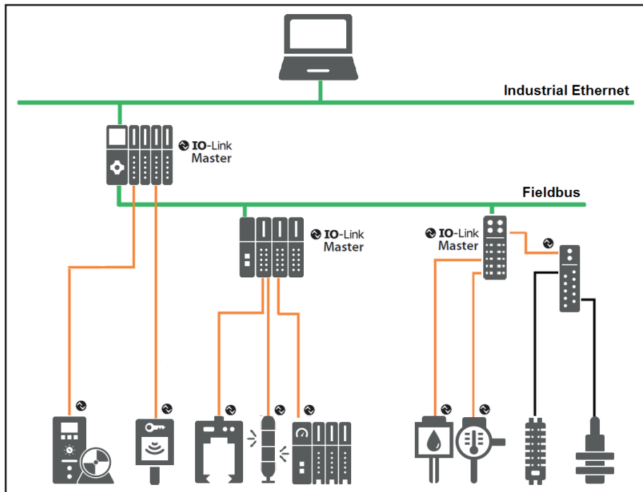
Figure 1: Example of system architecture with IO-Link
