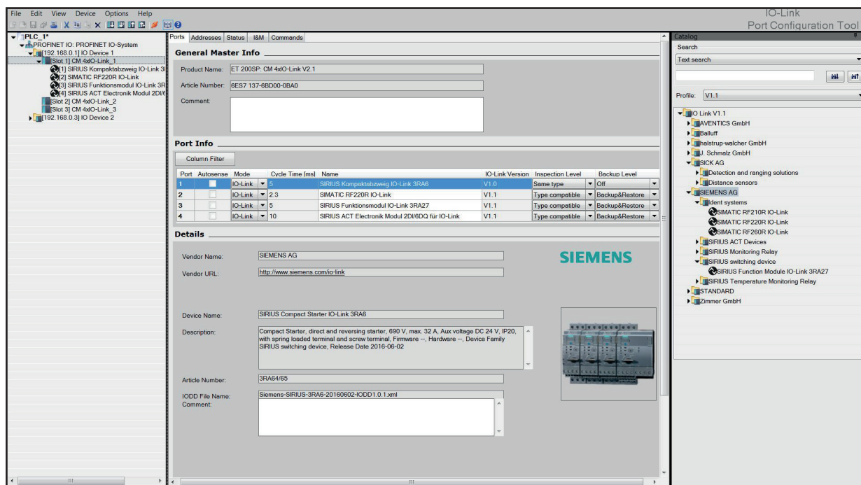
Figure 9: Configuration of an IO-Link master in the configuration tool
