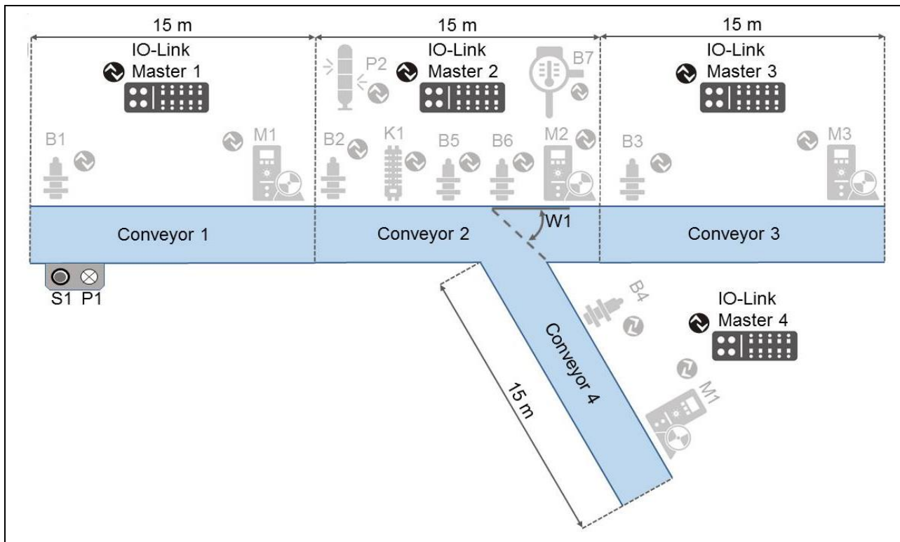
Figure 9: Placement of the IO-Link masters
