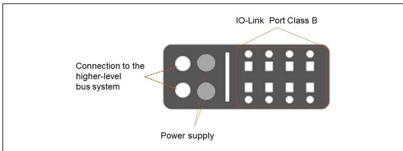
Figure 10: Connection diagram of the IO-Link master
